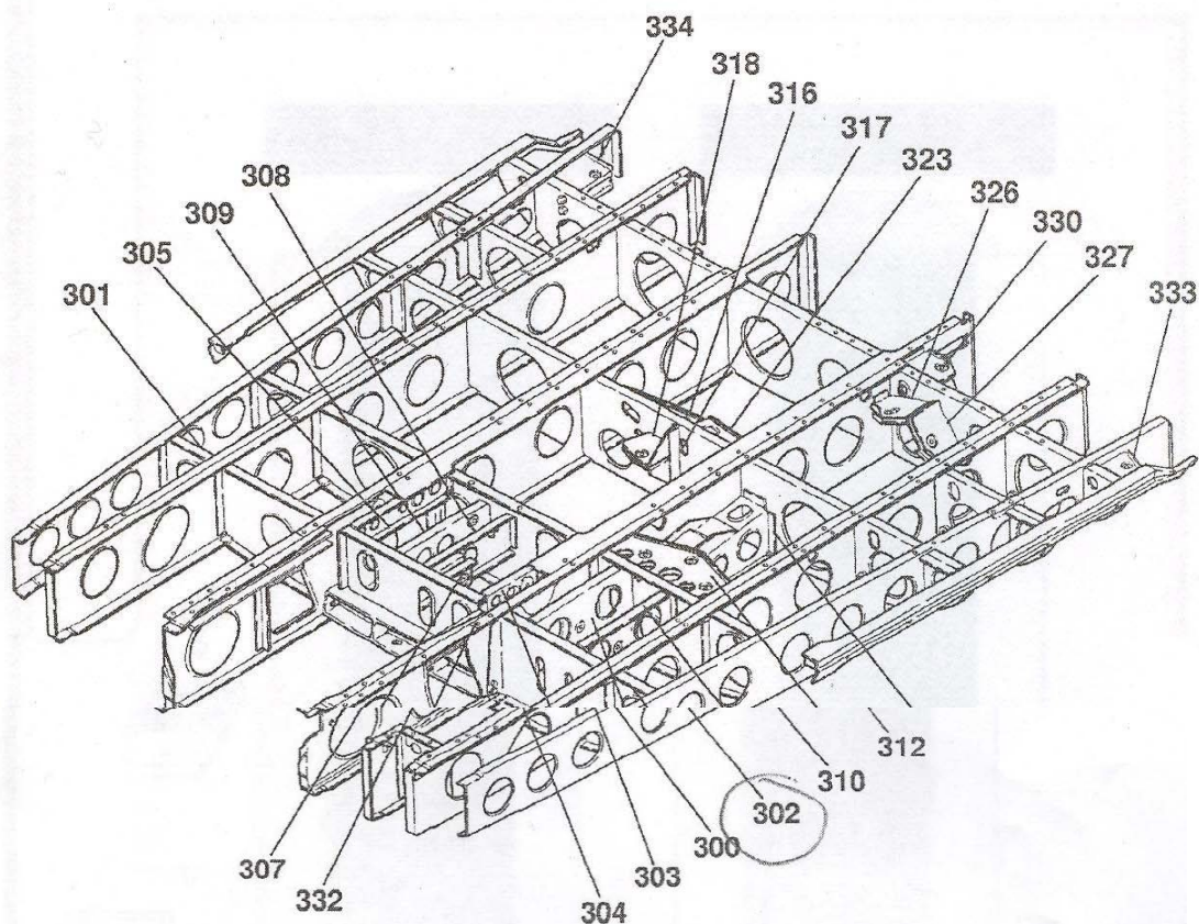
LOWER FORWARD FUSELAGE STRUCTURE FIGURE 01 (SHEET 5)
